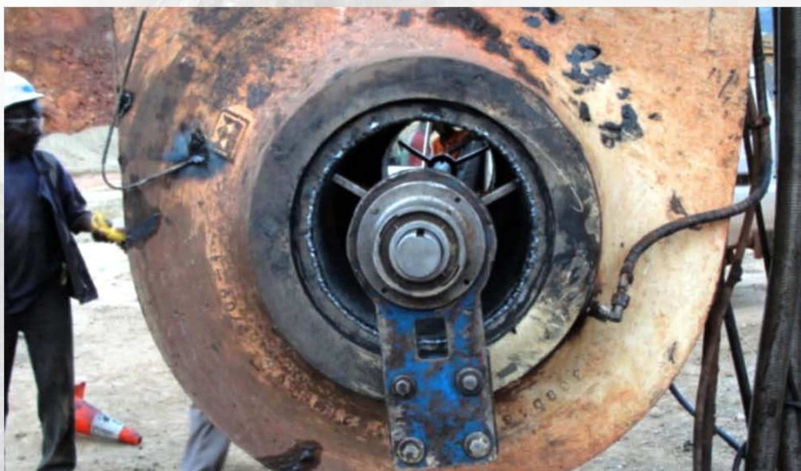
LINE BORING ON THE RH170 EXCAVATOR STICK.
